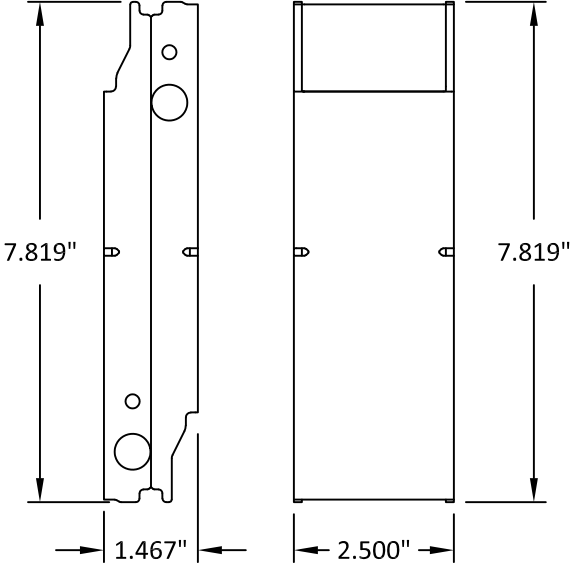
8" END MOUNT
