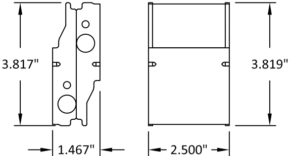
4" END MOUNT
