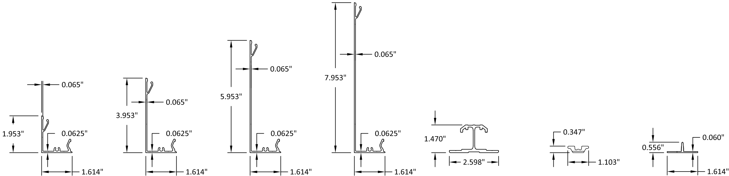
2" LINK & LOCK
