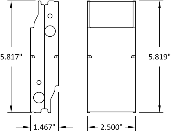
6" END MOUNT
