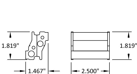
2" END MOUNT
